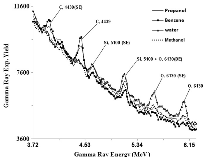
Fig. 5. Enlarged LaBr 3 :Ce detector prompt gamma ray spectra of benzene, propanol, water and methanol samples plotted over 3.72–6.15 MeV energy range showing carbon and oxygen peaks along with associated escape peaks.
