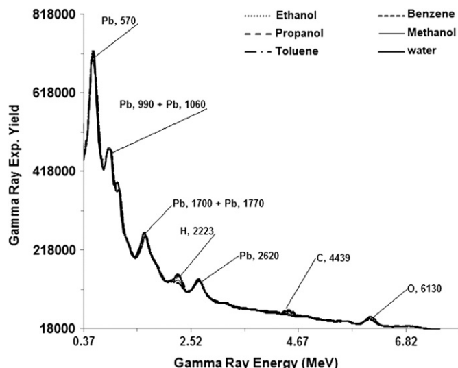
Fig. 6. Full prompt gamma ray spectra of 102 × 102 mm 2 (diameter × height) BGO gamma ray detector for benzene, ethanol, toluene, water and methanol samples.
