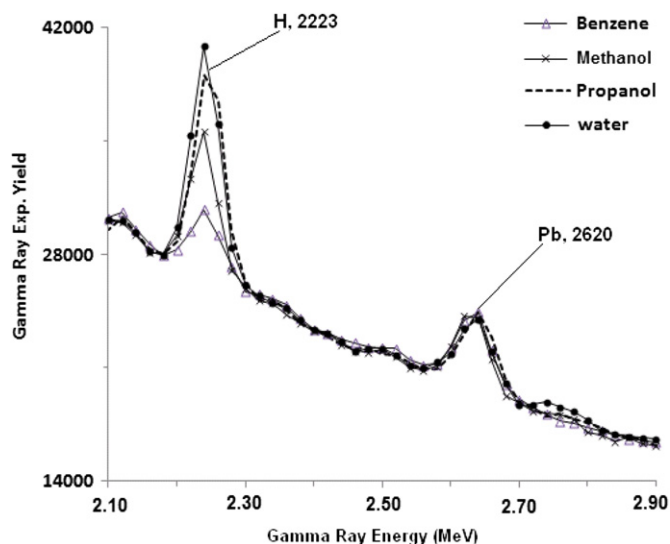
Fig. 4. Enlarged LaBr 3 :Ce detector prompt gamma ray spectra of benzene, activated propanol, water, methanol and lead shielding plotted over 2.10–2.90 MeV energy range showing hydrogen peak.
