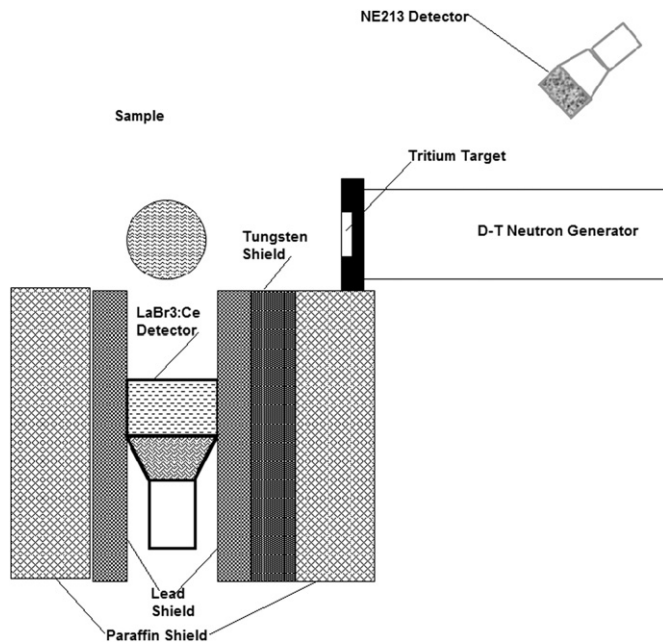
Fig. 1. Schematic of 14 MeV neutron-based setup used for measurement of hydrogen, carbon and oxygen concentration in bulk samples.
