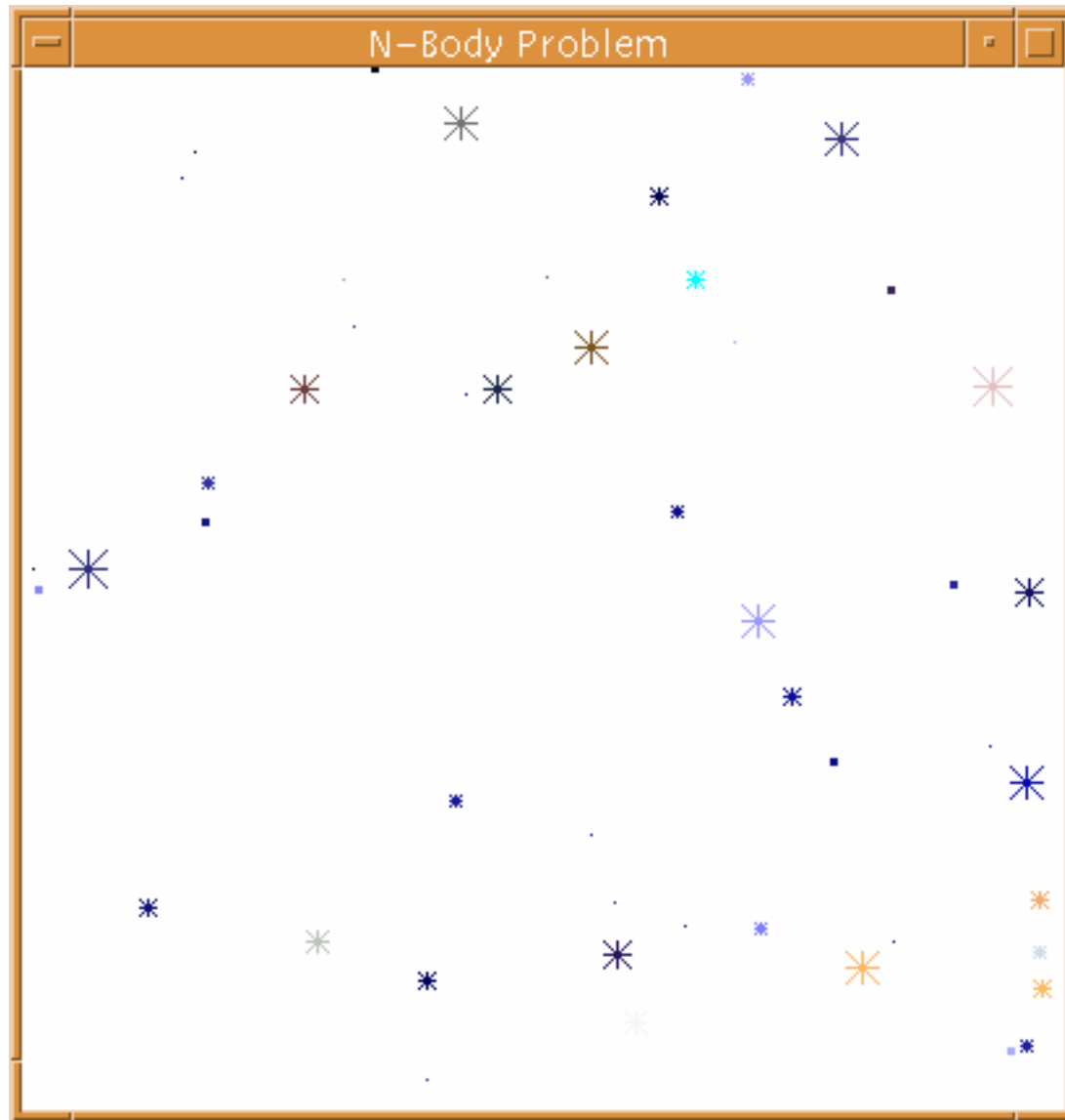
Astrophysical N -body simulation by Scott Linssen (undergraduate UNC-Charlotte student).
