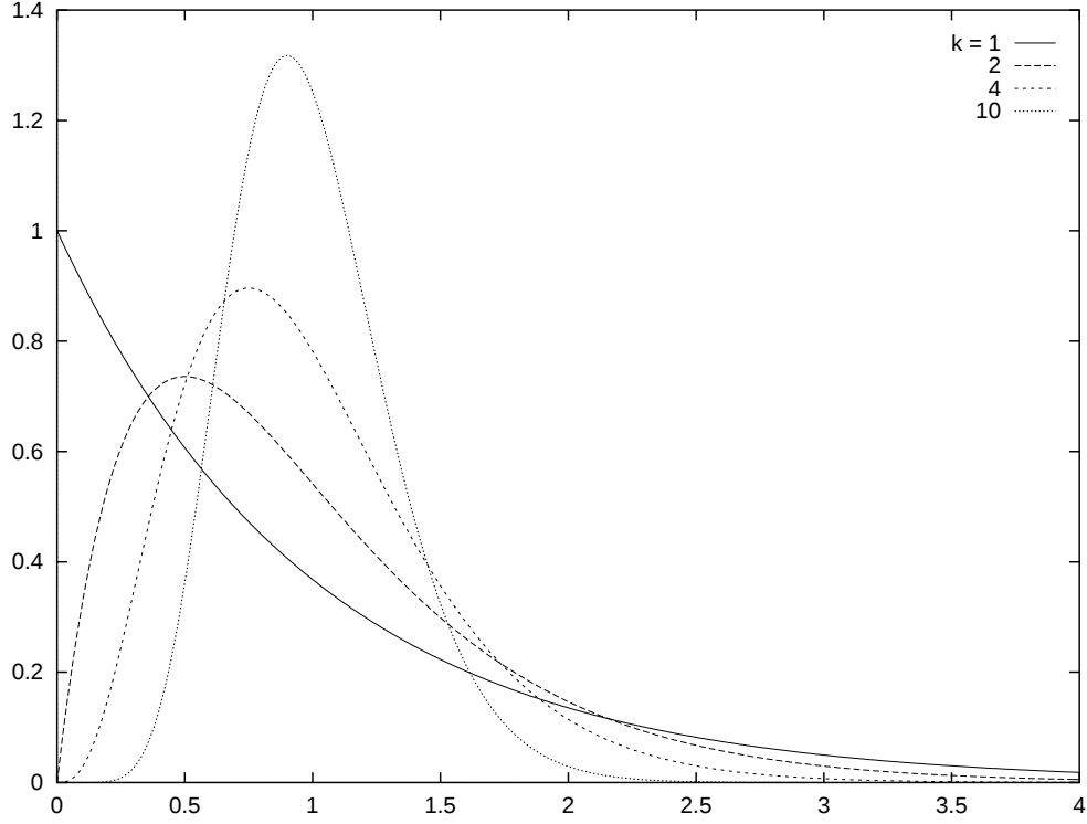
Figure 2.2: The density of the Erlang- k distribution with mean 1 for various values of k
