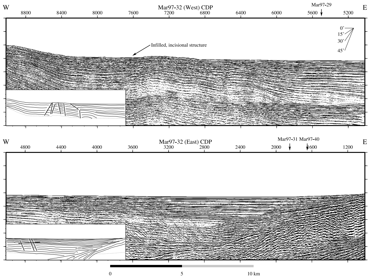
Figure 5. Sample migrated reflection profile from the eastern Sea of Marmara, showing dipping limestone basement from CDP 1000–3600, with unconformable deposits above. An infilled incisional canyon is highlighted at CDP 7600.
