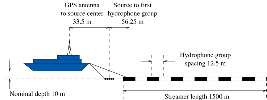
Figure 2. Schematic diagram of ship geometry during Marmara Sea cruise. All distances are measured in meters relative to the GPS antenna on the ship. The configuration shown is for a maximum streamer length of 1500 m.
