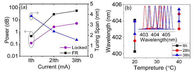
Fig. 3. (a) Comparison of the usable optical power of the violet tunable SIL-ECDL system with the FR LD power at three different injection currents along with the corresponding measured wavelength tuning window. (b) Temperature effect on the wavelength span of the violet tunable SIL-ECDL system at different injection currents. The inset of (b) depicts the normalized locked spectrums tunability at various current injections, and at 40°C.
