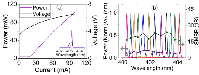
Fig. 2. (a) Room temperature L-I-V characteristics of the violet InGaN/GaN LD with the comparison between the FR and SIL spectrum at 25 mA in the inset. (b) Room temperature wavelength tunability of the violet tunable SIL-ECDL system at 21 mA alongside the corresponding extracted \Delta\lambda and the SMSR.
