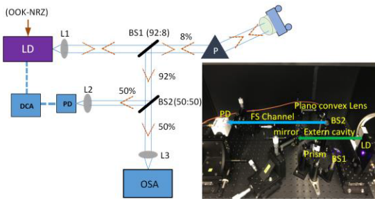
Fig. 1. The Schematic diagram of the SIL violet laser diode system with integrated transmission module. The inset show the photograph of the laboratory setup.
