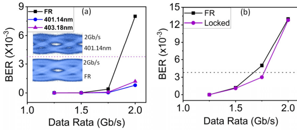
Fig. 5. BER versus the data rate of OOK-NRZ transmission experiments on (a) 0.4 m indoor free-space channel length at 35 mA and at two distinct tuned wavelengths of 401.14 and 403.18 nm (b) 0.8 m indoor free-space channel length at 50 mA and at a tuned wavelength of 401.14 nm. The unlocked FR LD results are also shown. Insets of (a) are the eye diagrams.
