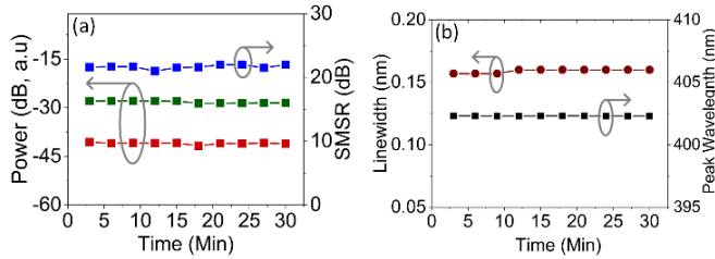
Fig. 4. Stability performance of the violet tunable SIL-ECDL system at a tuned wavelength of 402.29 nm in terms of (a) SMSR (blue), integrated power (green) and peak power (red), and (b) optical linewidth and peak wavelength.
