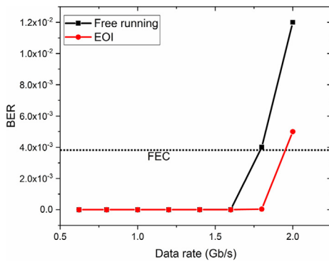
Fig. 9. Bit-error-rate of the red laser diode at different data rates in an EOI configuration 30 cm VLC link for an injection current of 115 mA and 190 mA for the slave and master laser diodes respectively. In this case, APD and standard laser diode mount are utilized in the system.
