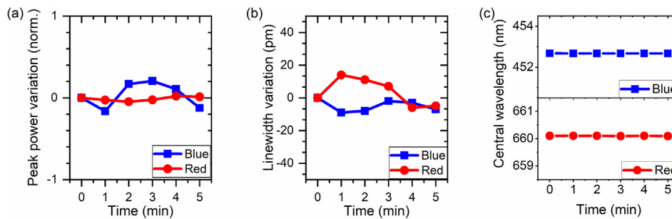
Fig. 6. Short-term stability test for blue and red lasers under EOI showing (a) peak power, (b) linewidth variation, and (c) peak wavelength. The values are taken for 5 min at a 1-minute interval. The linewidth of both the laser diodes has been normalized with respect to the first value to show a better comparison. The bias conditions of both the color systems follow that of Fig. 5.
