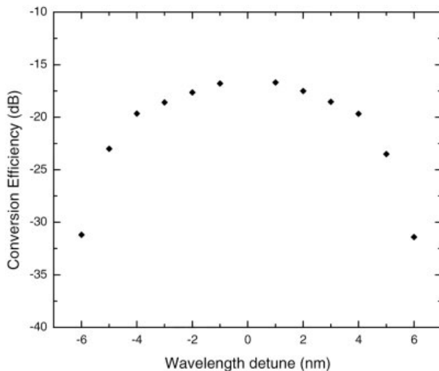
Figure 1 Measured conversion efficiency versus signal wavelength detuning relative to fixed pump wavelength of 1550 nm
