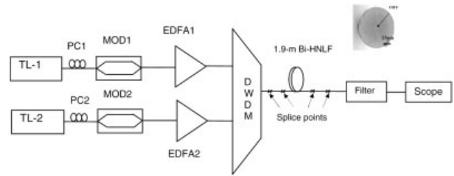
Figure 2 Experimental setup of the all-optical Bi-HNLF based on–off switch. TL: Tunable laser; PC: Polarization controller; MOD: Modulator; EDFA: Erbium-doped fiber amplifier; DWDM: Dense wavelength division multiplexer
