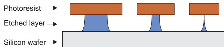
Figure 10. Isotropic etching versus linewidth.
