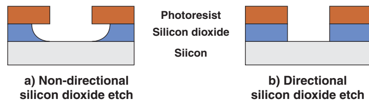
Figure 9. Isotropic versus anisotropic etching.
