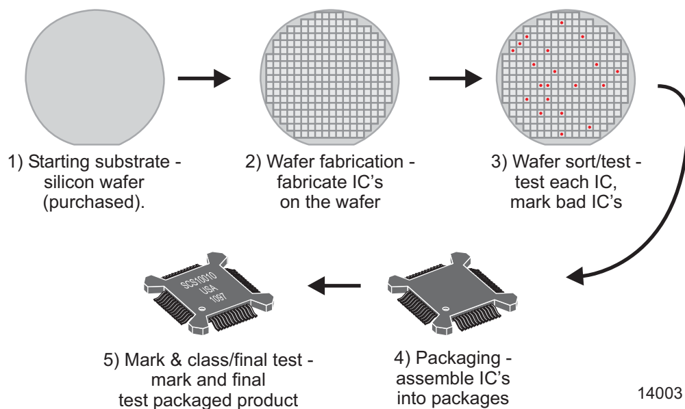
Figure 1. IC manufacturing.
