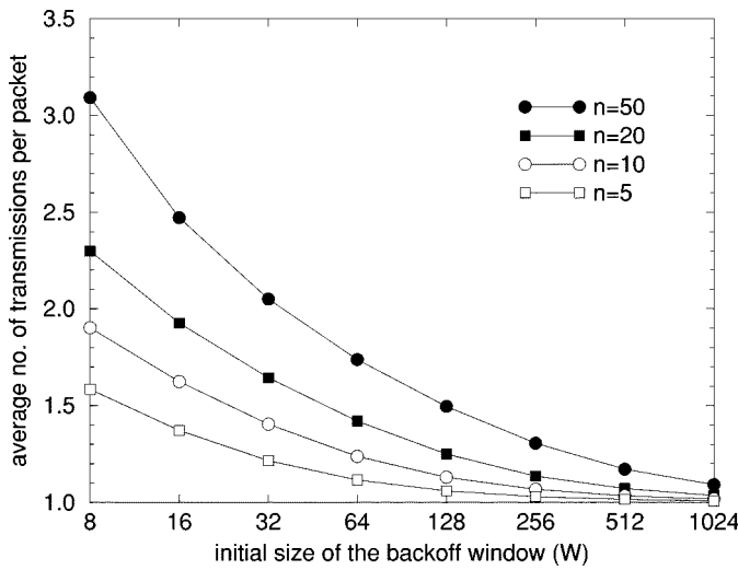
Fig. 14. Average number of transmissions per packet.
