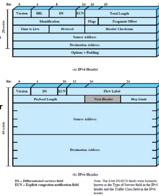
Figure 2.4 IP Headers
