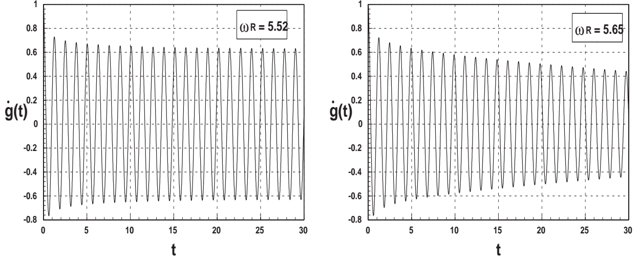
FIG. 4. The functions S(\omega) and \dot{g}(t) for the cases in which the pole is just below (left column) and just above (right column) the threshold frequency ( \omega_{th} = 5 ). In the left column, \omega_R = 5.52 , \omega_p = 4.98083 and Z = 0.63845 while in the right column \omega_R = 5.65 , \omega_p = 5.07373 and Z = 0.69959 . The numerical parameters are \eta = 3.0 and \omega_c = 55 , with \Gamma/\omega_p \approx 0.005 .
