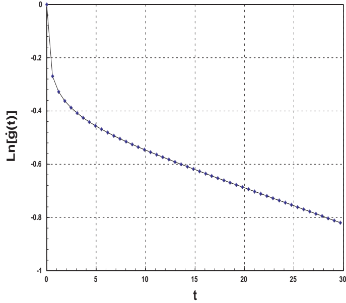
FIG. 5. The logarithm of the maxima of \dot{g}(t) vs t for \eta = 3.0 and \omega_c = 55 , \omega_{th} = 5 , \omega_R = 5.52 , \omega_p = 4.98083 and Z = 0.63845 , corresponding to the right column of fig.4.
