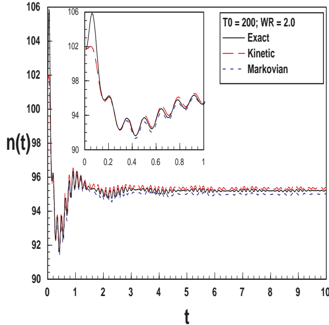
FIG. 2. The expectation value of the particle occupation number given by eq.(2.2) for \Omega = \omega_p for the case in which the pole is below threshold for particle temperature T_0 = 200 and bath temperature T = 100 . The pole is at \omega_p = 1.95719 and Z = 0.95621 . The numerical parameters are \eta = 0.85 , \omega_c = 45 , \omega_{th} = 5 and \omega_R = 2 .
