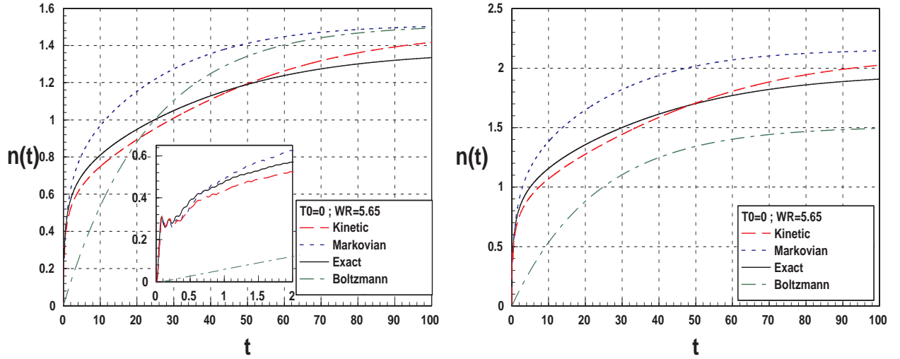
FIG. 7. The expectation value of the number operator eq.(2.2) for the same values of the parameters as for the right column in figure(4)(quasiparticle pole above threshold), \eta = 3.0 and \omega_c = 55 , \omega_{th} = 5 , \omega_R = 5.65 , \omega_p = 5.07373 and Z = 0.69959 . The temperature of the bath is T = 10 and zero initial particle temperature ( T_0 = 0 ), the exact, Markovian and kinetic curves have been divided by the wave function renormalization Z in the rightmost figure. The insert in the left figure shows the early time behavior.
