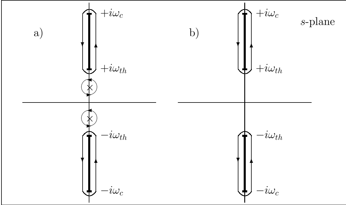
FIG. 1. The complex contour used to evaluate g(t) for the cases in which a) the pole is below the threshold and b) the pole is above threshold.
