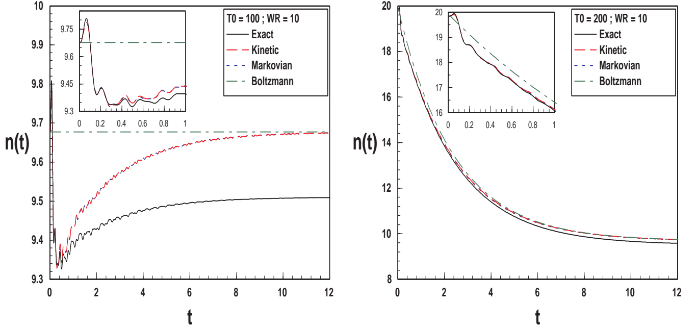
FIG. 3. The expectation value of the particle occupation number given by eq.(2.2) for \Omega = \omega_p for the case in which the pole is above threshold for particle temperatures T_0 = 100 and 200 and bath temperature T = 100 . The pole is at \omega_p = 9.83397 and Z = 0.99631 . The numerical parameters are \eta = 0.85 , \omega_c = 45 , \omega_{th} = 5 and \omega_R = 10 , resulting in \Gamma/\omega_p \approx 0.02 .
