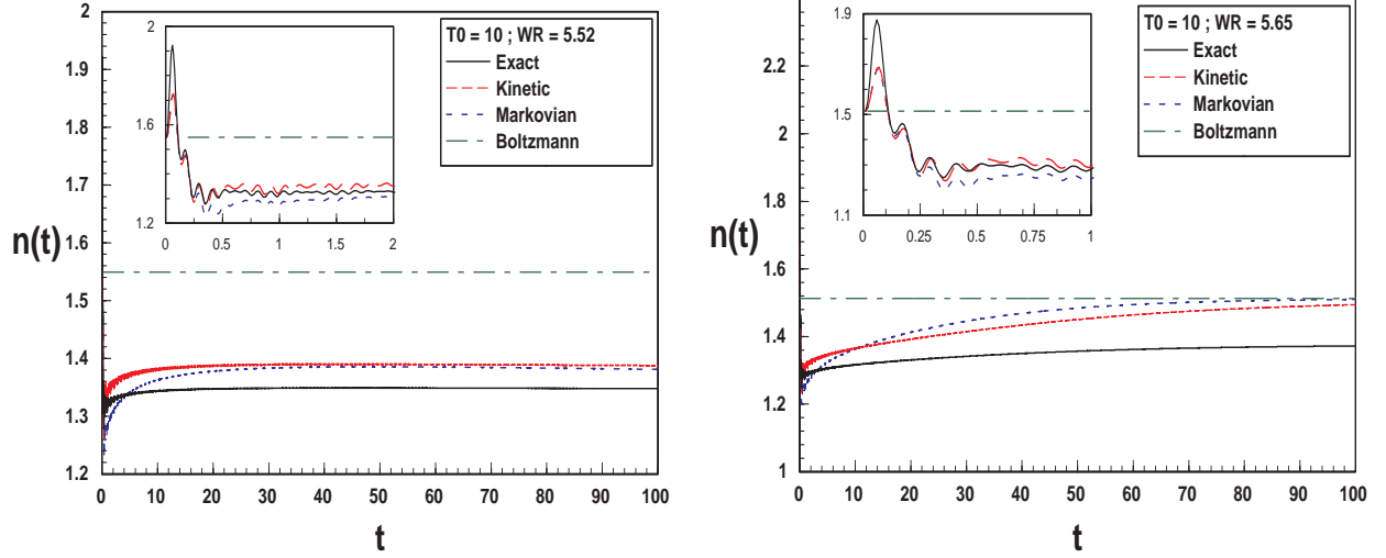
FIG. 6. The expectation value of the number operator eq.(2.2) for the same values of the parameters as in figure(4)(left figure corresponds to pole below threshold and right figure to the pole above threshold) for the case of equal particle and bath temperature T_0 = T = 10 . The insert shows the early time behavior.
