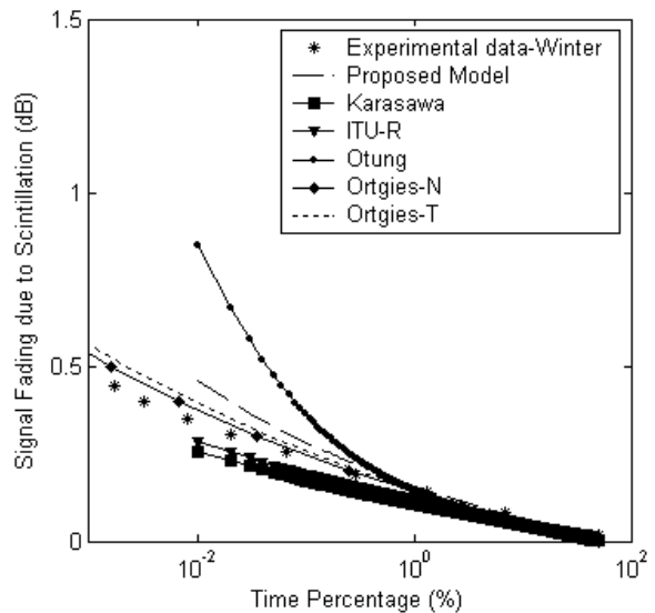
Figure 4: Comparison between new proposed model for scintillation fade and experimental
