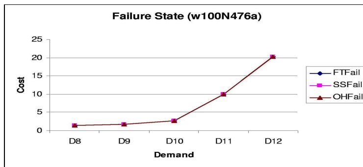
Figure 12: Comparison of FT, SS, and OH in the Failure state for w100N476a Network.
