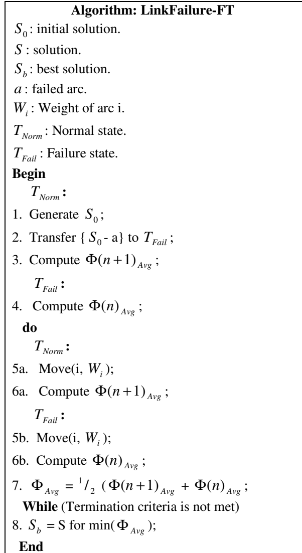
Figure 1: Structure of the LinkFailure – FT algorithm.
