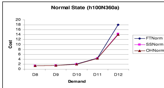
Figure 3: Cost Comparison FT, SS and OH in the Normal state for h100N360a Network.
