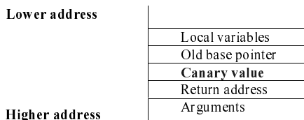
Figure 3. The StackGuard stack frame
