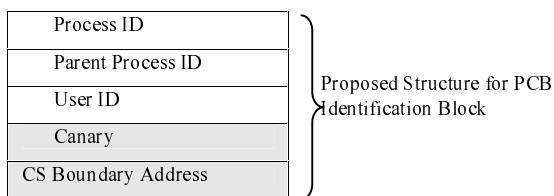
Figure 5. Modified process control block
