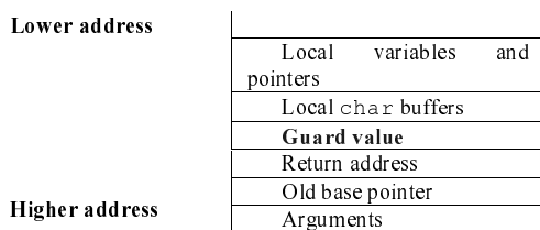
Figure 4. The ProPolice stack frame
