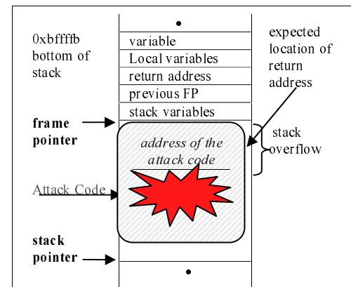
Figure 2b. Stack view after attack
