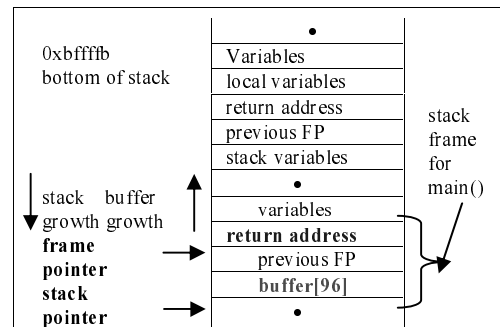
Figure 2a. Stack view before attack
