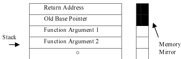
Figure 6. proposed memory architecture
