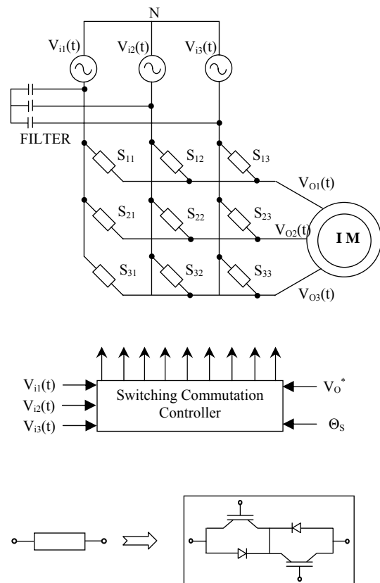
Figure 1. The topology of three-phase to three-phase matrix converter and the configuration of bi-directional switch.
