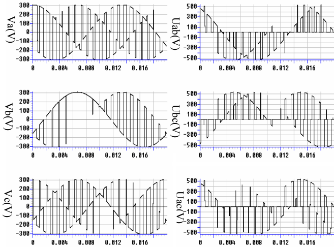
Figure 4. voltages waveforms v_a , v_b , v_c , u_{ab} , u_{bc} and u_{ac} , for: f_s=1 kHz, f_i=50 Hz, f_o=25 Hz, q=0.57
