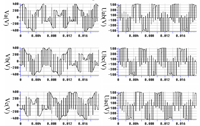
Figure 7. voltages waveforms, v_a , v_b , v_c , u_{ab} , u_{bc} and u_{ac} , for: f_s=2 kHz, f_i=50 Hz, f_o=200 Hz, q=0.866
