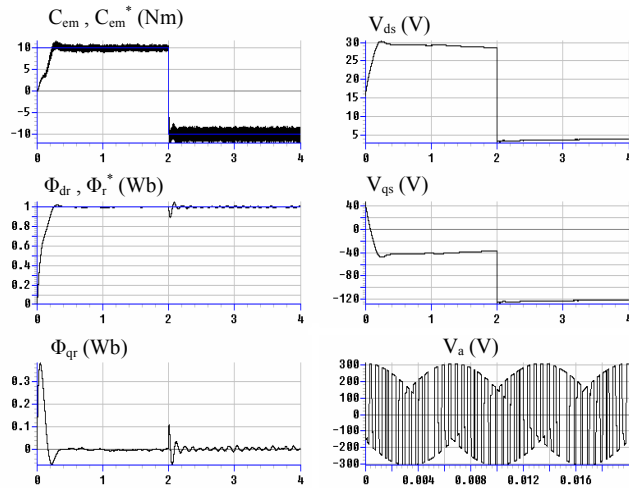
Figure 8. Decoupling flux - torque at f_s=2 kHz.
