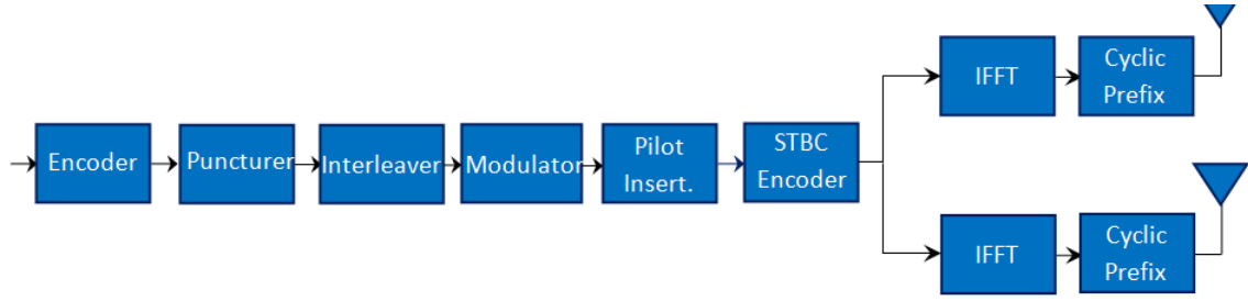
Fig. 1. STBC MIMO OFDM Transmitter.
