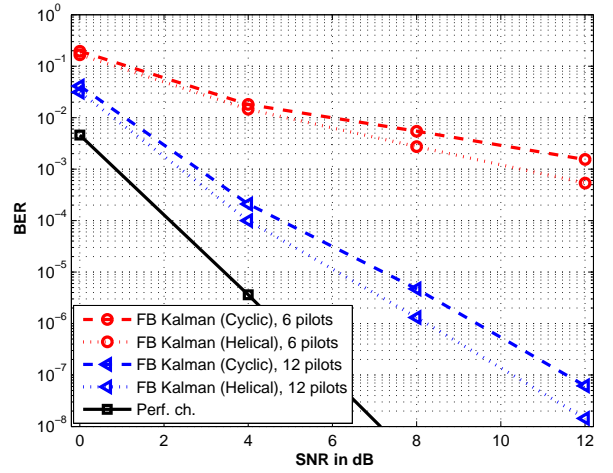
Fig. 4. Performance using different number of pilots
