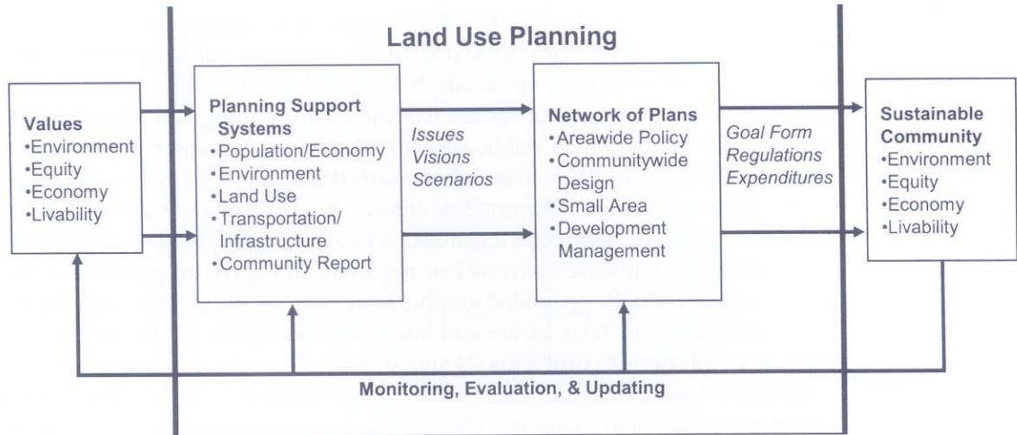
Fig. 1-1 Conceptual framework of land use planning.
