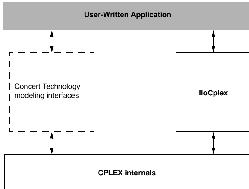
Figure 5.1 A View of ILOG CPLEX in ILOG Concert Technology
