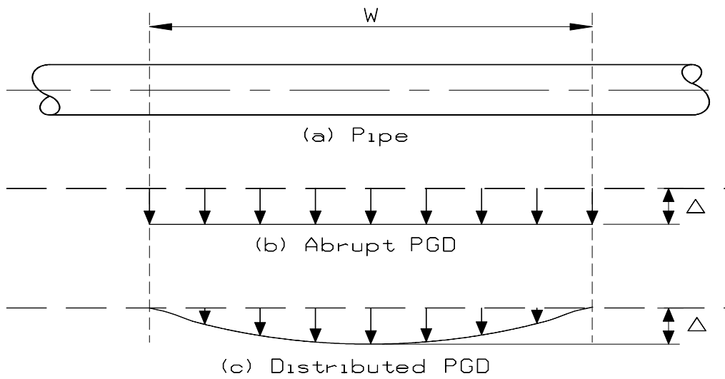
Figure 11.2-3 Transverse PGD With Spatial Extent W and Amount of Movement \Delta
