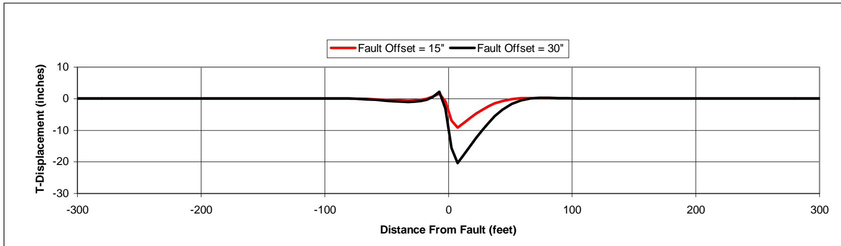
Figure 8.3-4(d) Displacement in Transverse Soil Springs Along the Pipeline
