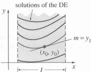
FIGURE 1.8 Solution of second-order IVP
