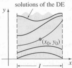
FIGURE 1.7 Solution of first-order IVP
