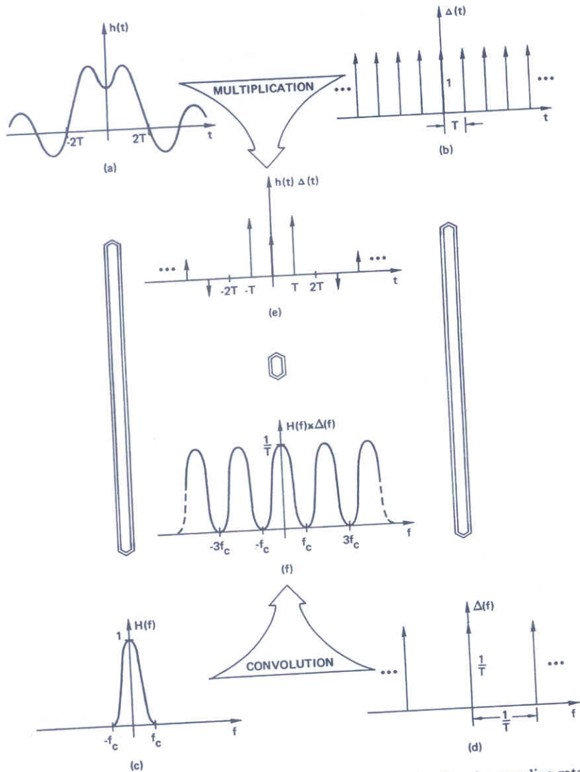
Figure 5.6 Fourier transform of a waveform sampled at the Nyquist sampling rate.
