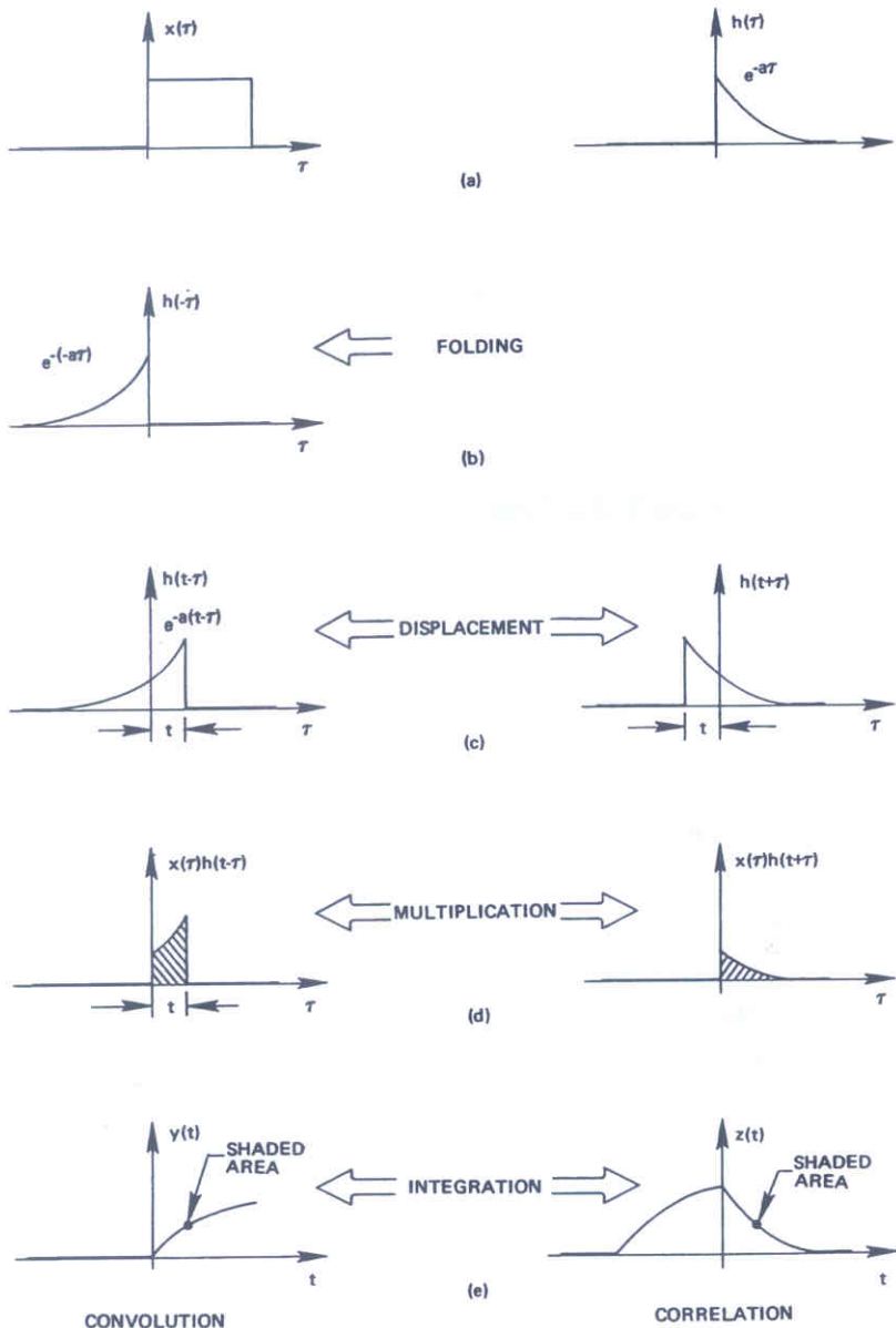
Figure 4.12 Graphical comparison of convolution and correlation.
