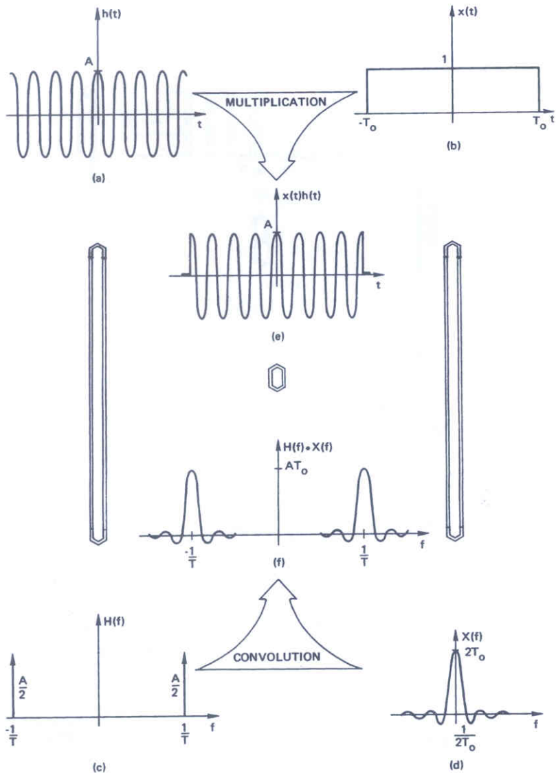
Figure 4.11 Graphical example of the frequency-convolution theorem.
