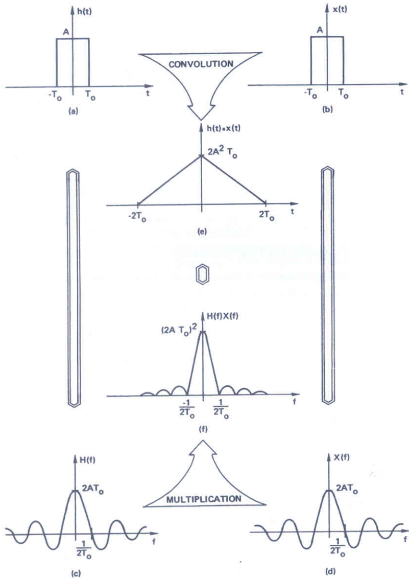
Figure 4.9 Graphical example of the convolution theorem.
