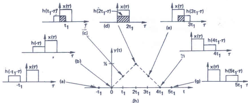
Figure 4.3 Graphical example of convolution; t_1 = 1/2 .
