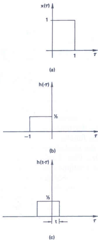
Figure 4.2 Graphical illustration of folding and displacement operations.
