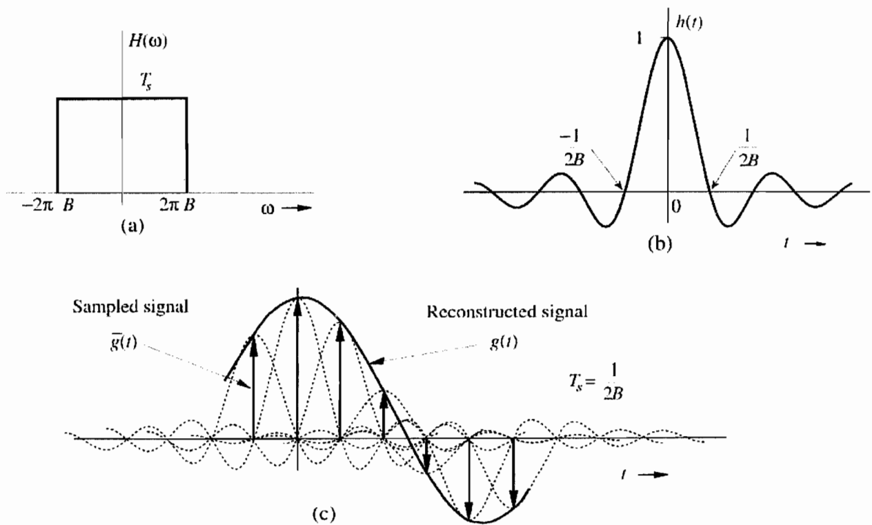
Figure 6.3 Ideal interpolation.
