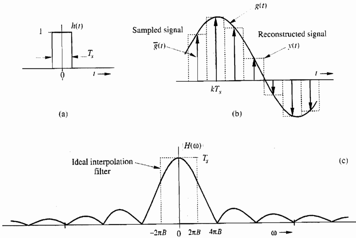
Figure 6.2 Simple interpolation using zero-order hold circuit.
