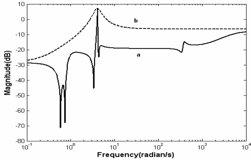
Fig.3 (a) Plot of \sup \left| \tilde{P}(j\omega) / P_{nom}(j\omega) - 1 \right| , (b) fitted W_2 function
