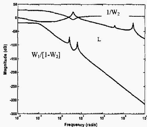
Fig.3 The open-loop function and the frequency boundaries
