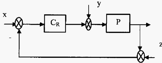
Fig.2 The plant-controller configuration for robust design
