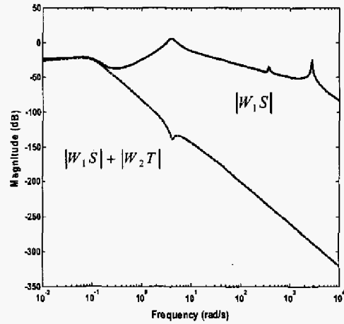
Fig.4 Convergence of robust performance and stability indices
