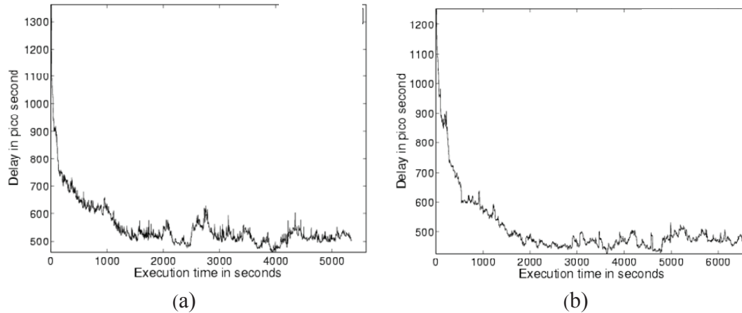
Figure 10. Delay versus execution time: (a) OFSE and (b) AFSE
