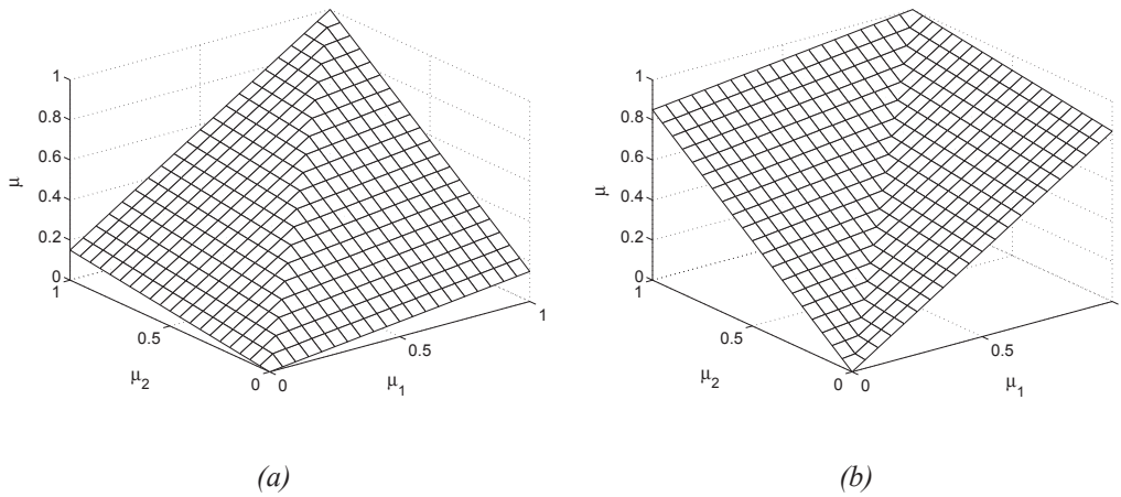
Figure 2. (a) Fuzzy AND-like OWA operator; (b) Fuzzy OR-like OWA operator
