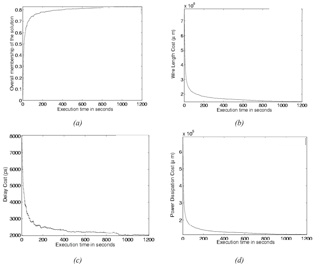
Figure 11. (a) Overall membership (b) wire-length cost (c), circuit delay, and (d) power cost versus execution time in seconds for circuit S15850 using FFSE.
