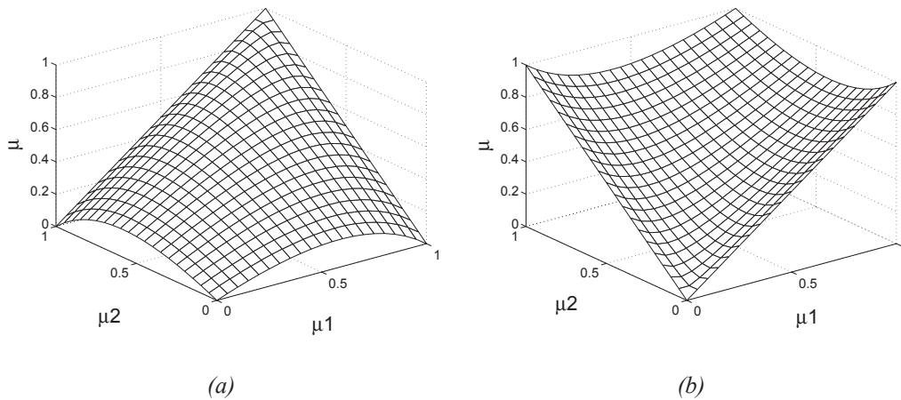
Figure 3. (a) AND-Like Fuzzy Aggregation; (b) OR-Like Fuzzy Aggregation
