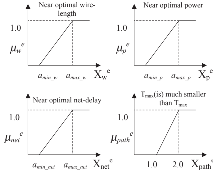
Figure 6. Membership functions used in fuzzy evaluation
