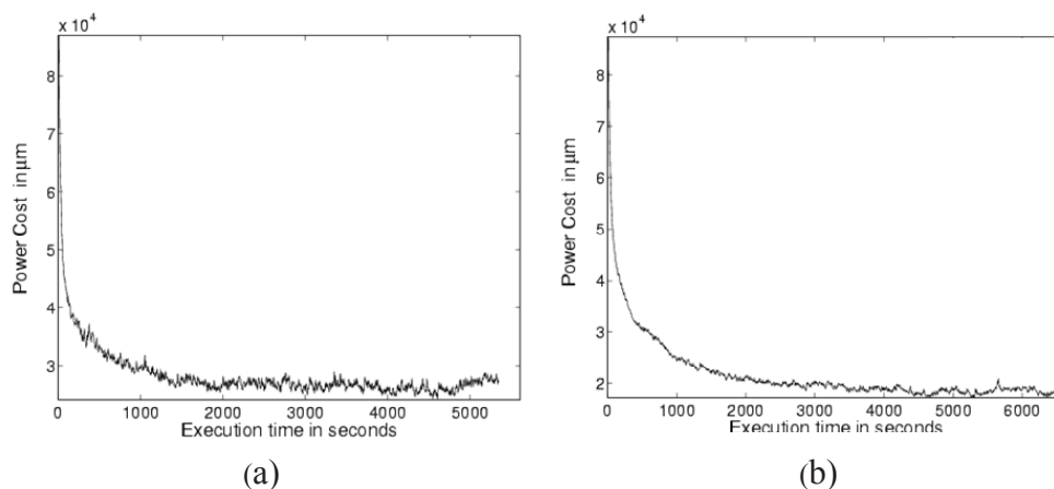
Figure 9. Power-cost versus execution time: (a) OFSE and (b) AFSE
