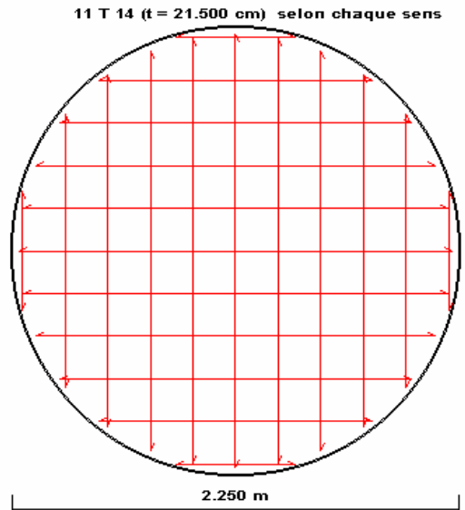
Fig.4: Design of footings
