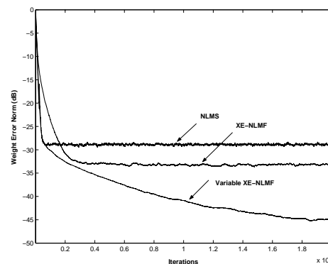
Fig. 3. Convergence performance for the variable XE-NLMF algorithm, the XE-NLMF algorithm ( \alpha=0.5 ) and the NLMS algorithm in AWGN environment.
