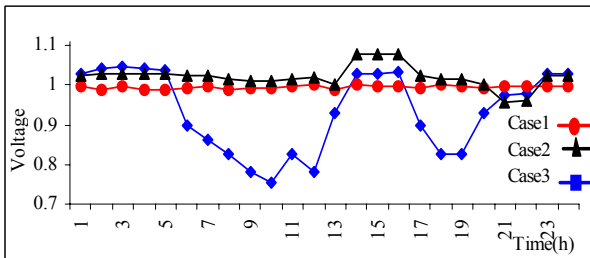
Fig.5. Voltage variations of bus19 over a day
