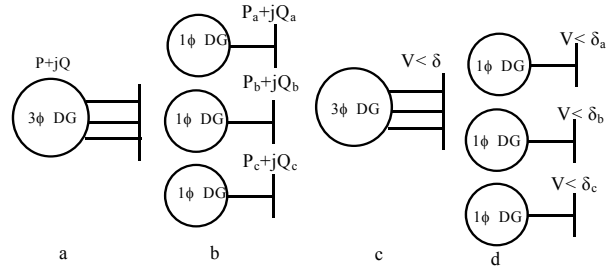
Fig.1. Models of DGs
