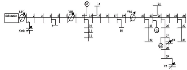
Fig.2 Single Line Diagram
