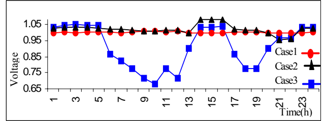
Fig.7. Voltage variations of bus34 over a day
