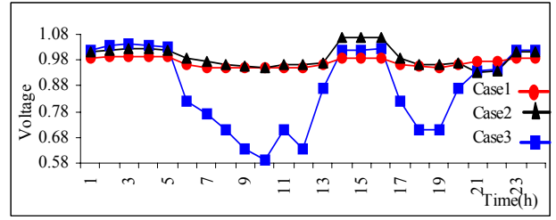
Fig.6. Voltage variations of bus21 over a day
