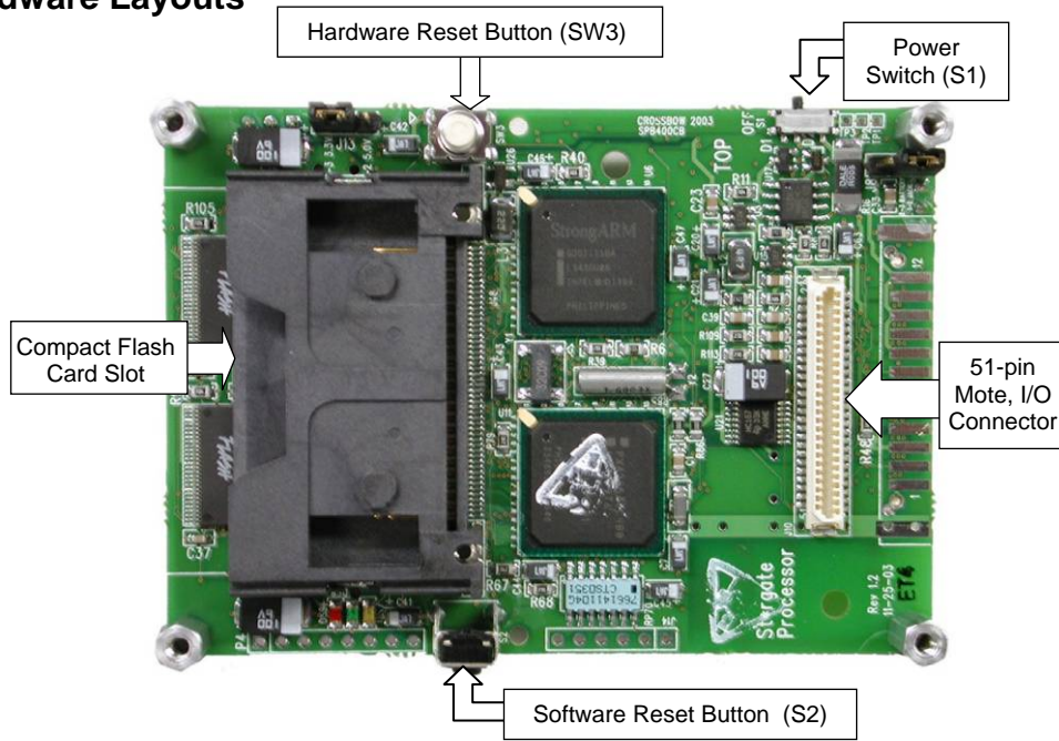
Figure 2. SPB400CB Processor Board (Top View)
