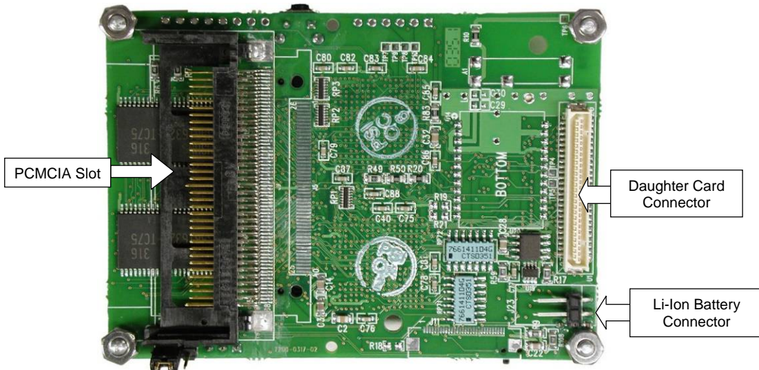
Figure 3. SPB400CB Processor Board (Bottom View)
