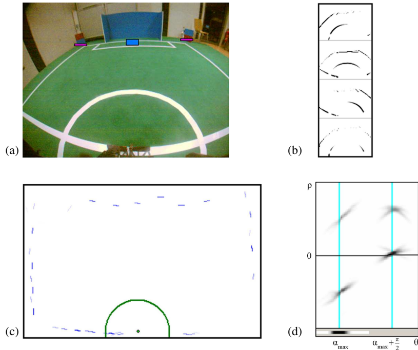
Fig. 2. Illustration of the extraction of lines: The robot’s current field of view can be seen in image (a). The four small images (b) show responses of four oriented line detectors. Image (c) depicts the extracted line segments projected into the egocentric space. The center circle is detected and removed. Image (d) shows the representation of the line segments in the Hough space, where the major orientation \alpha_{max} is estimated and the main lines are detected.
