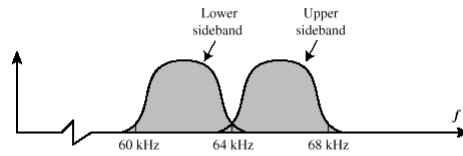
(b) Spectrum of s_1(t) for f_1 = 64 kHz
