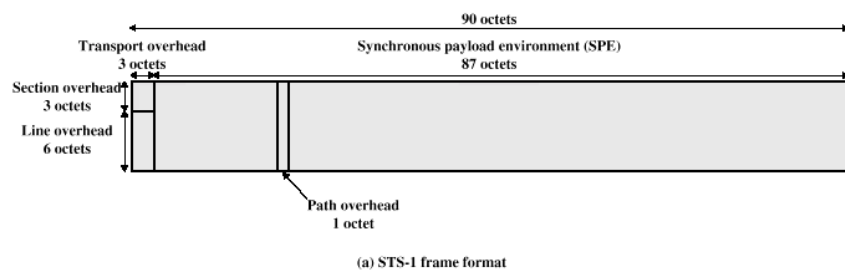
(a) STS-1 frame format
