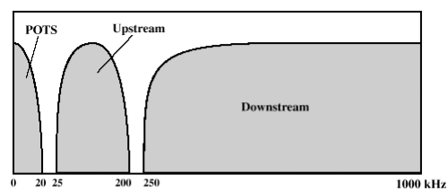
(a) Frequency-division multiplexing
