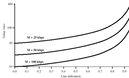
(a) Mean delay versus utilization
