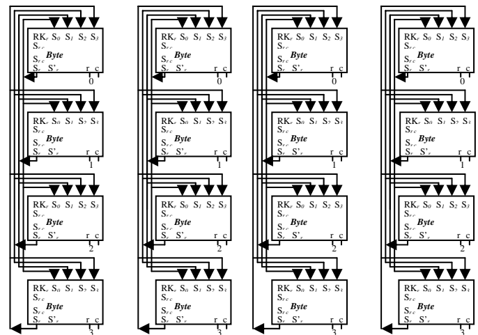
Figure 6 – Mix-Columns Operation Connections
