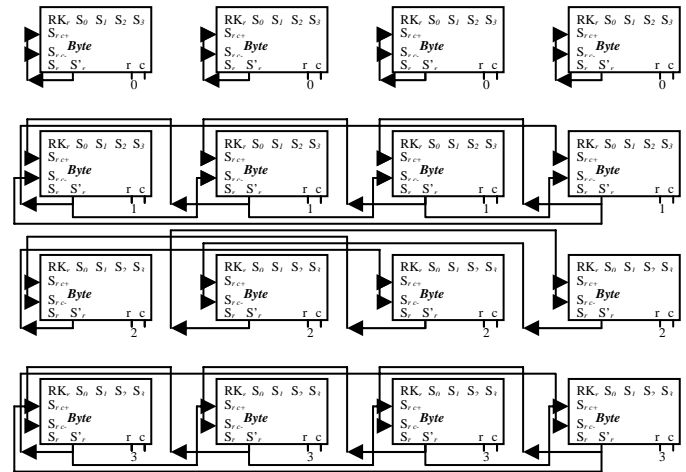
Figure 5 – Mix-Columns Operation Connections
