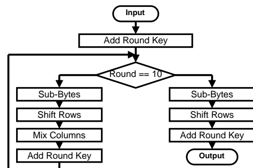
Figure 1 – AES Algorithm
