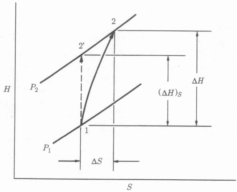
Figure 7.9: Adiabatic compression process.
