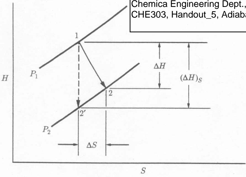
Figure 7.7: Adiabatic expansion process in a turbine or expander.
