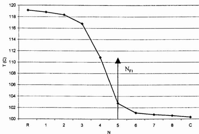
Figure 6. Column 3 temperature and composition profiles.
