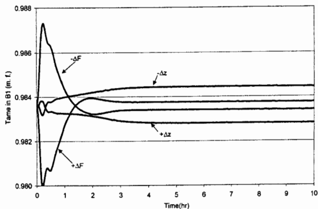
Figure 12. Column 1 TAME purity.
