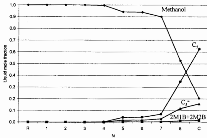
Figure 5. Column 2 temperature and composition profiles.
