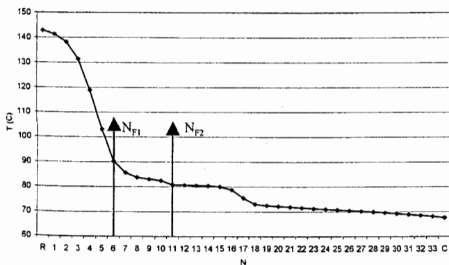
Figure 4. Column 1 temperature and composition profiles.
