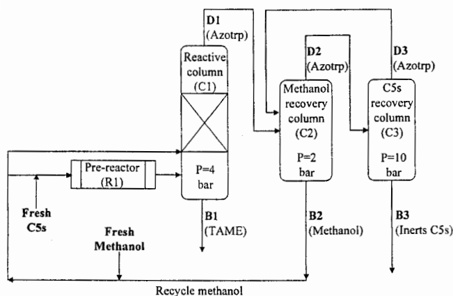
Figure 2. Flowsheet sketch.
