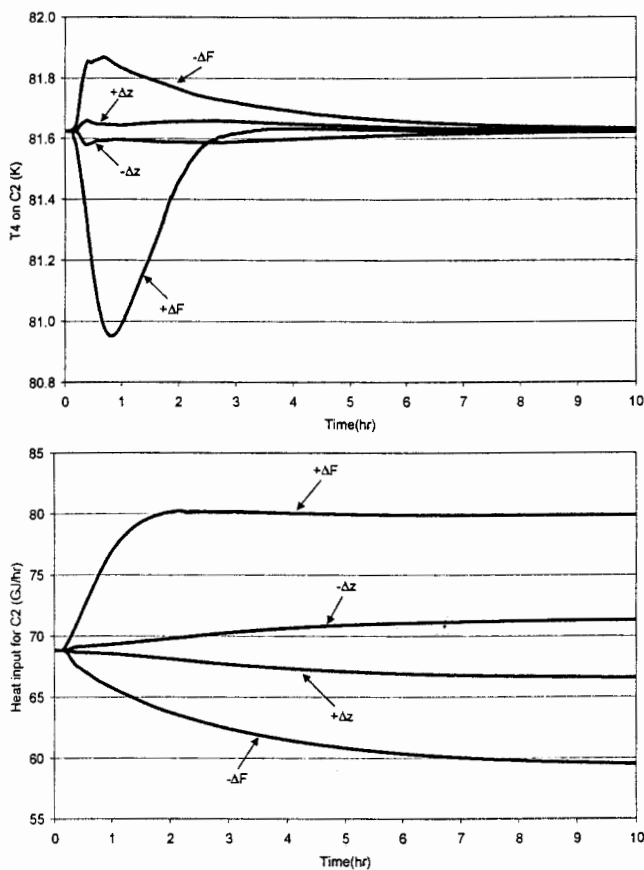
Figure 13. Column 2 temperature controller.
