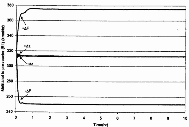
Figure 15. Fresh methanol feed.
