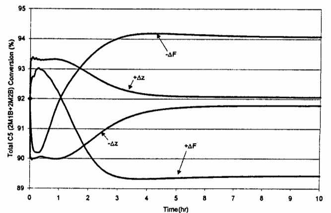
Figure 17. Overall conversion.
