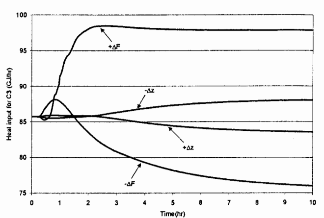
Figure 16. Column 3 temperature controller.
