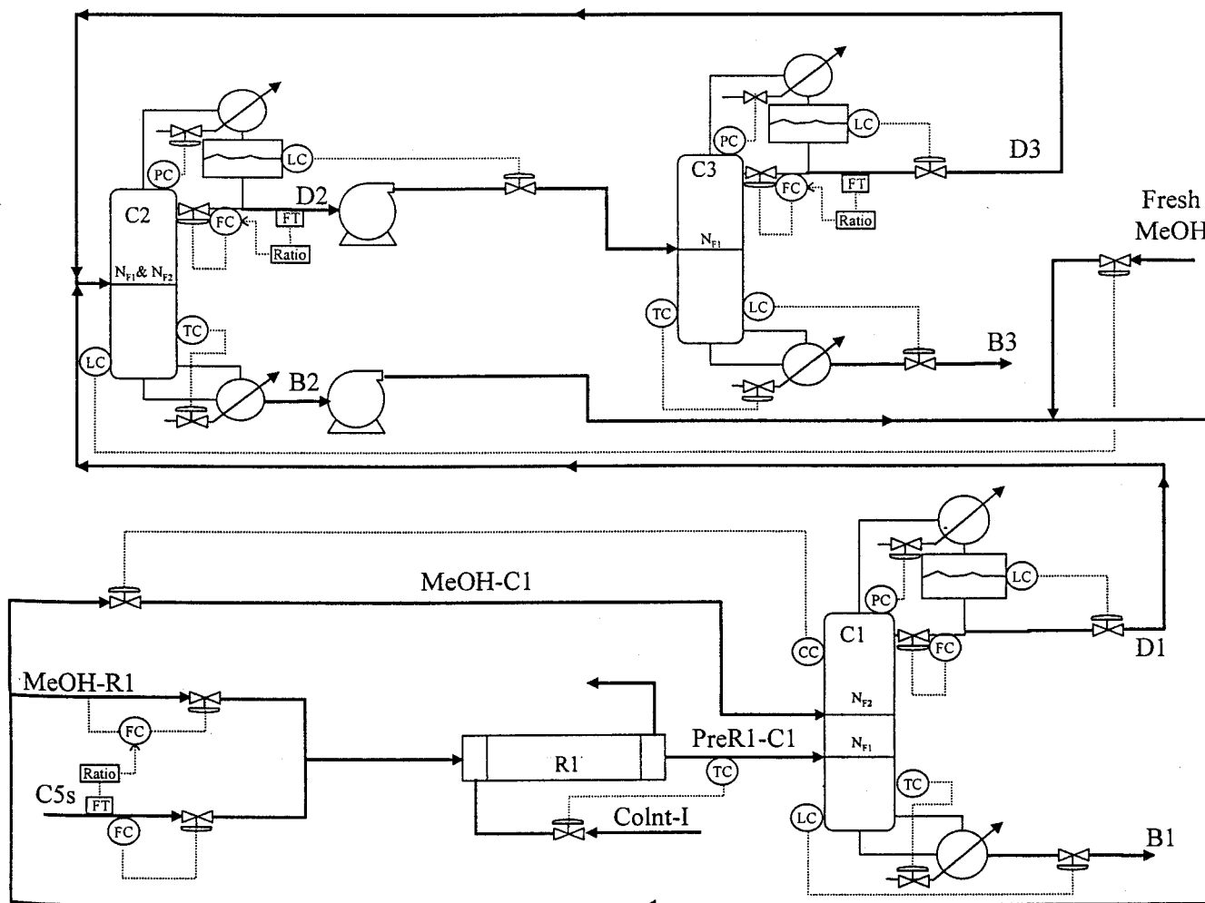
Figure 9. Control structure.
