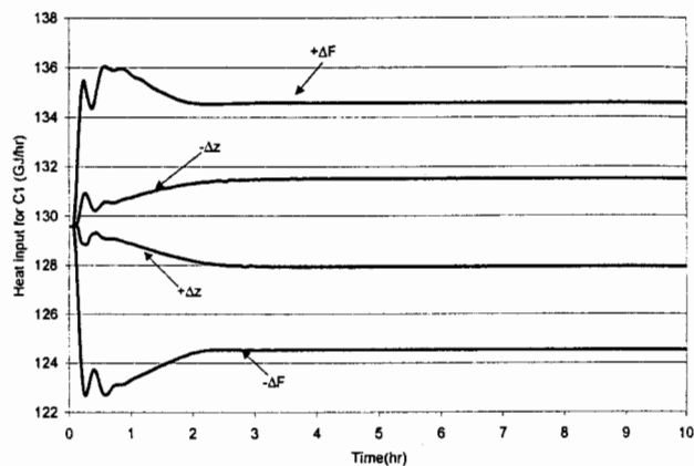
Figure 11. Column 1 temperature controller.
