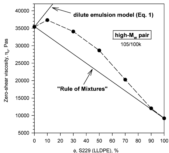
Fig. 8 \eta_o(\phi) obtained with Carreau model from \eta'(\omega) data in Fig. 5 for blends of S229 (butene LLDPE) and S216 (LDPE), (high- M_w pair, T_{\text{test}} = 190^\circ\text{C} , \dot{\gamma}^\circ = 10\% , T_{\text{mix}} = 190^\circ\text{C} )
