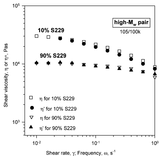
Fig. 7 Comparison of \eta(\dot{\gamma}) and \eta^*(\omega) for blends of S229 (butene LLDPE) and S216 (LDPE), (high- M_w pair, T_{\text{test}} = 190^\circ\text{C} , \dot{\gamma}^\circ = 10\% , \dot{\gamma} = 0.01\text{--}1\text{ s}^{-1} , T_{\text{mix}} = 190^\circ\text{C} )
