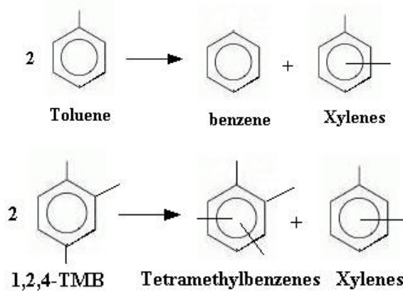
Fig. 1. Reactions occurring during Transalkylation reaction of 1,2,4-Triemethylbenzene with Toluene
