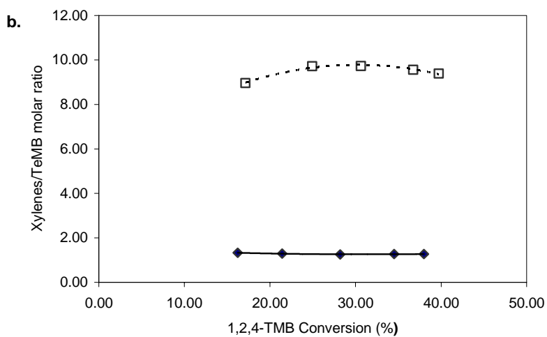
Fig. 8. X/TeMB ratio comparisons between 1,2,4-TMB reaction alone (◆) and transalkylation reaction of 1,2,4-TMB with Toluene (□) at a) 400°C; b) 500°C
