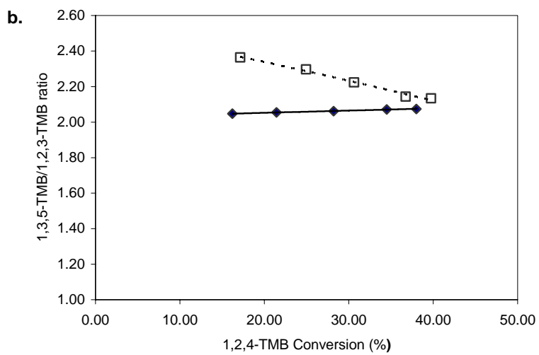
Fig. 6. 1,3,5-TMB/1,2,3-TMB ratio comparisons between 1,2,4-TMB reaction alone (◆) and transalkylation reaction of 1,2,4-TMB with Toluene (□) at a) 400°C; b) 500°C
