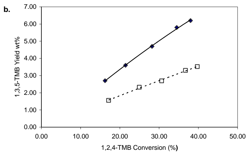
Fig. 7. 1,3,5-TMB Yield comparisons between 1,2,4-TMB reaction alone (◆) and transalkylation reaction of 1,2,4-TMB with Toluene (□) at a) 400°C; b) 500°C
