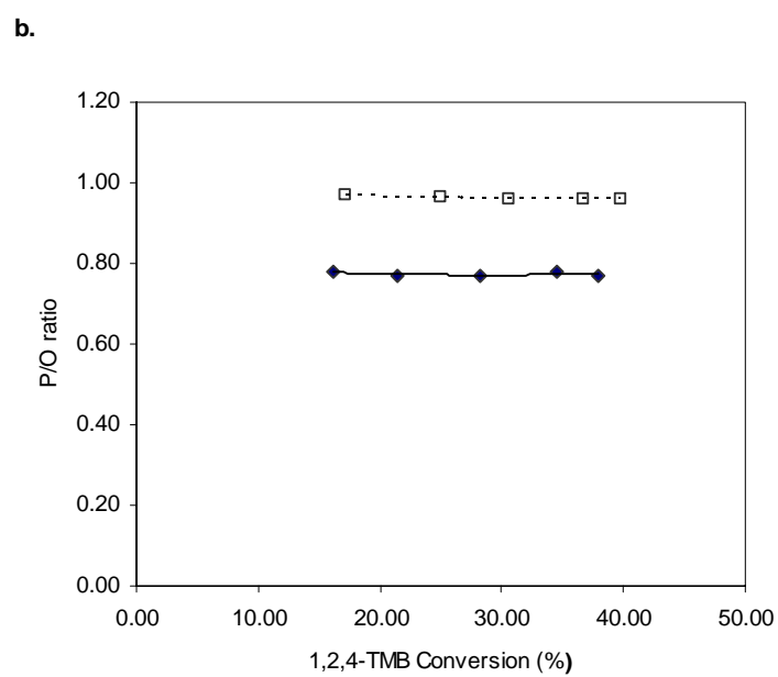
Fig. 5. P/O ratio comparisons between 1,2,4-TMB reaction alone (◆) and transalkylation reaction of 1,2,4-TMB with Toluene (□) at a) 400°C; b) 500°C
