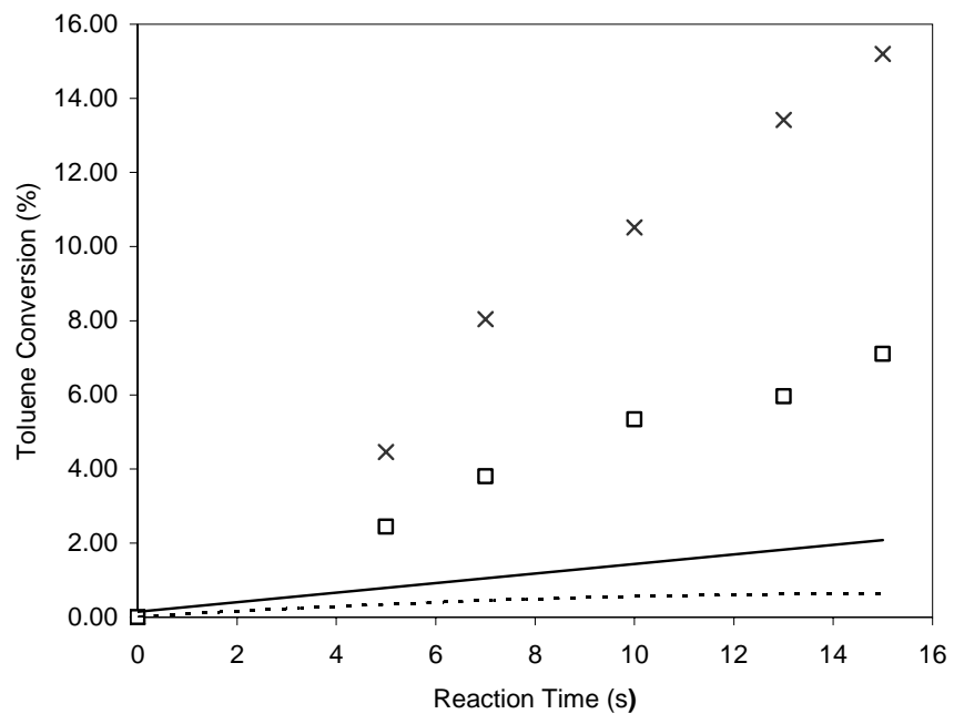
Fig. 3. Reactivity comparisons between Toluene reaction alone (----) 400°C and (—) 500°C; and transalkylation reaction of 1,2,4-TMB with Toluene (□) 400°C and (x) 500°C
