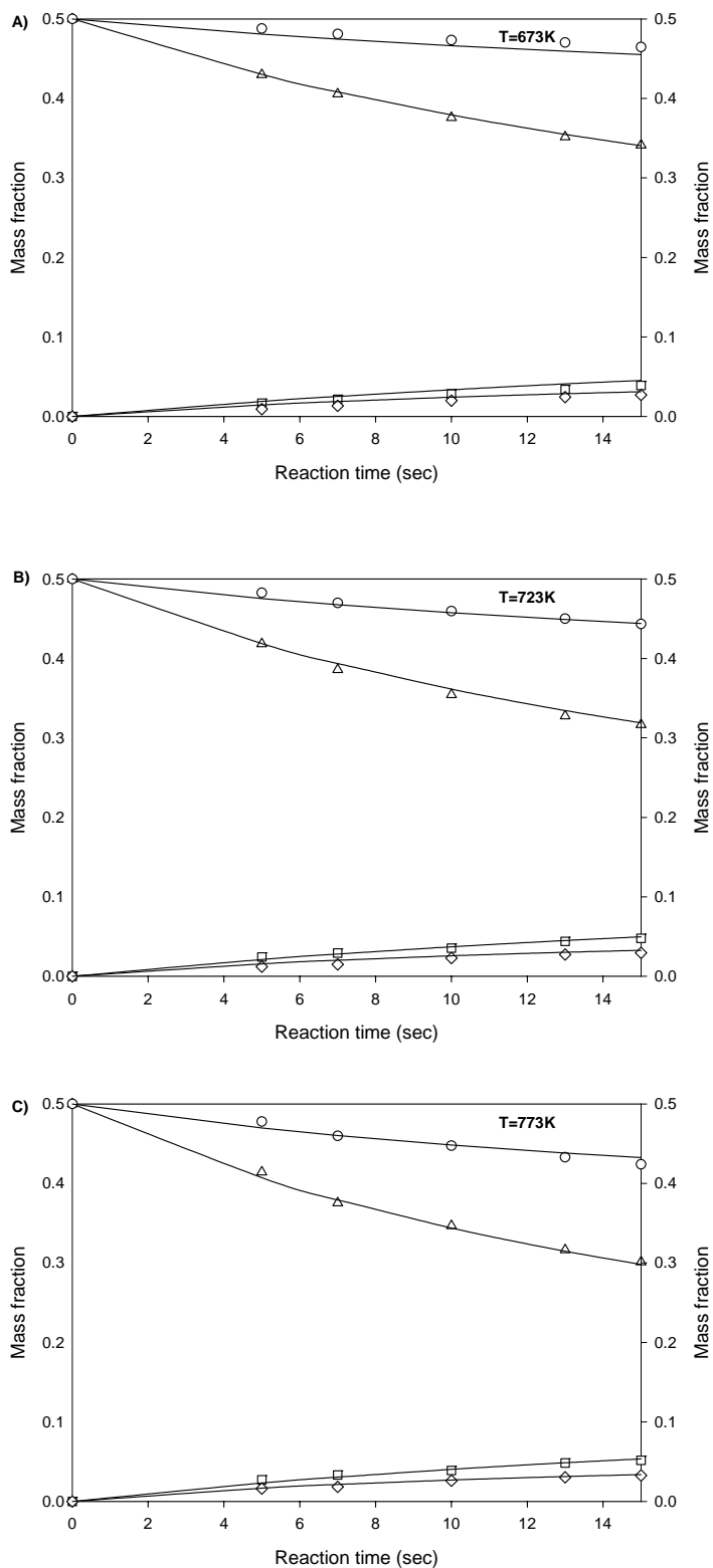
Fig. 9: Comparison between experimental results and numerical simulations (—) based on reaction network (Scheme 1) for 1,2,4-TMB transalkylation reaction with Toluene. (A) T = 673 K; (B) T = 723 K; (C) T = 773 K. (○) Toluene; (Δ) 124-TMB; (□) Isomerization Products [1,2,3 & 1,3,5-TMB]; (◇) Disproportionation Product [TeMB]
