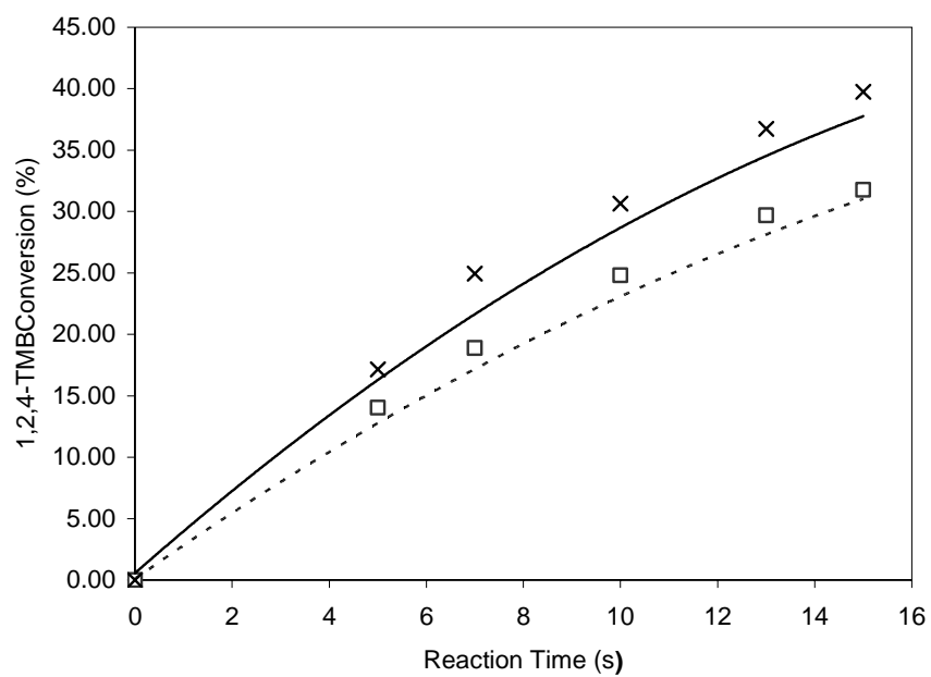
Fig. 2. Reactivity comparisons between 1,2,4-TMB reaction alone (----) 400°C and (—) 500°C; and transalkylation reaction of 1,2,4-TMB with Toluene (□) 400°C and (x) 500°C
